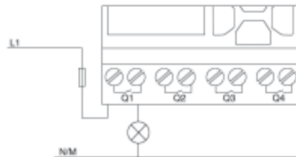
Fig 2.10 Relay Output
