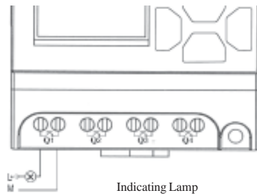
Fig. 2.1 Transistor Output
