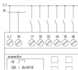
Fig 2.7 AC Type
